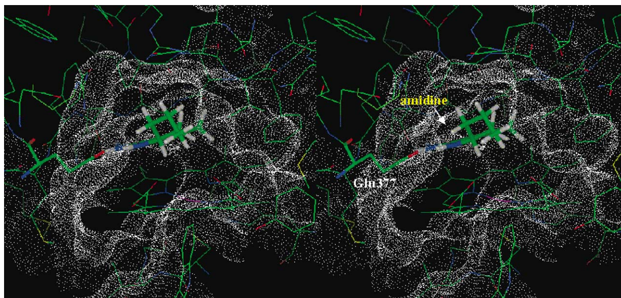
Figure 1. Stereo view of a docking model of compound 10 with human iNOS (PDB code 2NSI).
