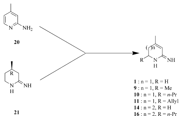
Chart 1. Molecular design of 5,6-dihydropyridin-2(1 H )-imine ( 1 and 9–11 ) and 1,5,6,7-tetrahydro-2 H -azepin-2-imine ( 14 and 16 ).
