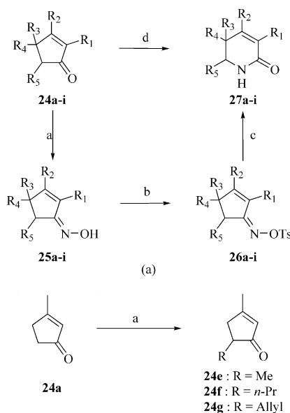
Scheme 1. Synthesis of 5,6-dihydropyridin-2(1 H )-imines ( 1 and 2 ) and 3,6-dihydropyridin-2(1 H )-imines ( 3 and 4 ). Reagents: (a) Li, liquid NH 3 , THF/EtOH, −78°C; (b) NH 4 Cl; (c) H 2 O (64–79%).
