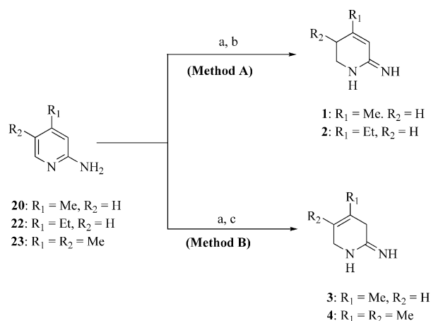
Scheme 1. Synthesis of 5,6-dihydropyridin-2(1 H )-imines ( 1 and 2 ) and 3,6-dihydropyridin-2(1 H )-imines ( 3 and 4 ). Reagents: (a) Li, liquid NH 3 , THF/EtOH, −78°C; (b) NH 4 Cl; (c) H 2 O (64–79%).
